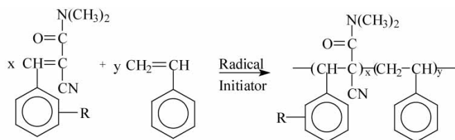
Sch. 1. ST-TSE copolymer synthesis. (R=3-benzyloxy, 4-benzyloxy, 3-ethoxy-4-methoxy, 3-bromo-4-methoxy, 5-bromo-2-methoxy, 2-chloro-6-fluoro).
